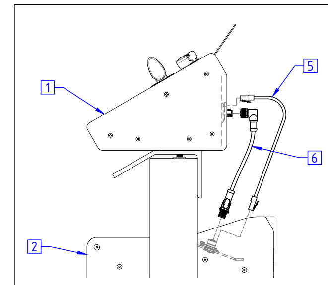
DETAIL A. CONSOLETTA CABLES SCALE 1:6
