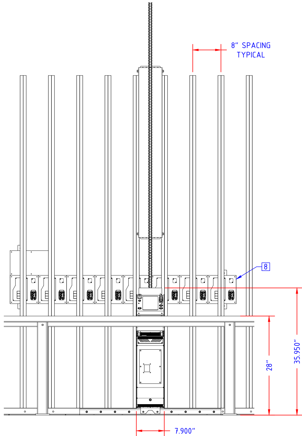
1. FRONT VIEW SCALE 1:16
